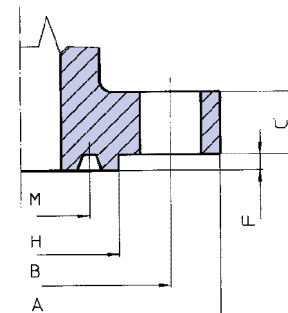
RING JOINT FACE
