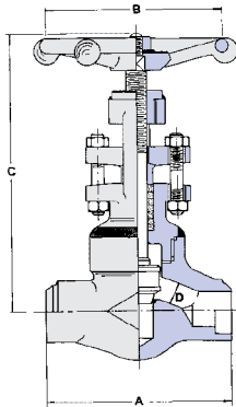
RATINGS: Carbon Steel - 11110 p.s.i. @ 100°F
