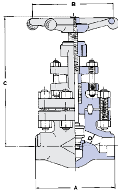
RATINGS: Carbon Steel - 11110 p.s.i. @ 100°F
