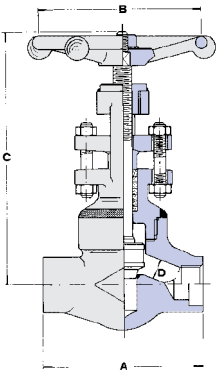
RATINGS: Carbon Steel - 1975 p.s.i. @ 100°F
