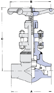
RATINGS: Carbon Steel - 3705 p.s.i. @ 100°F
