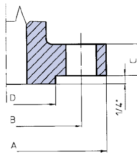
RAISED FACE 600 & 1500 lb
