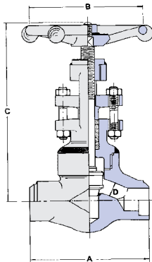
RATINGS: Carbon Steel - 6170 p.s.i. @ 100°F
