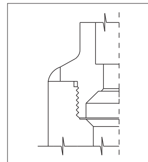
Screwed and Seal Weld "L"
