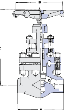
RATINGS: Carbon Steel - 6170 p.s.i. @ 100°F
