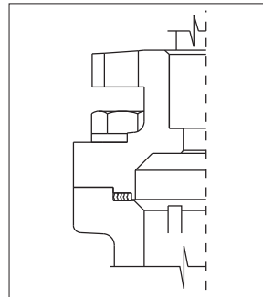
Gasket Joint
