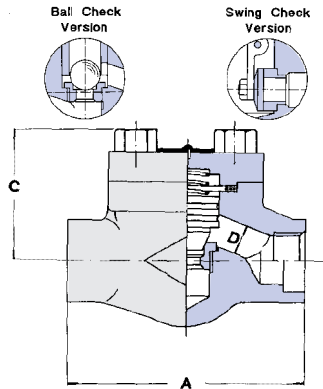
RATINGS: Carbon Steel - 1975 p.s.i. @ 100°F
